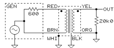
TEST CIRCUIT 3
